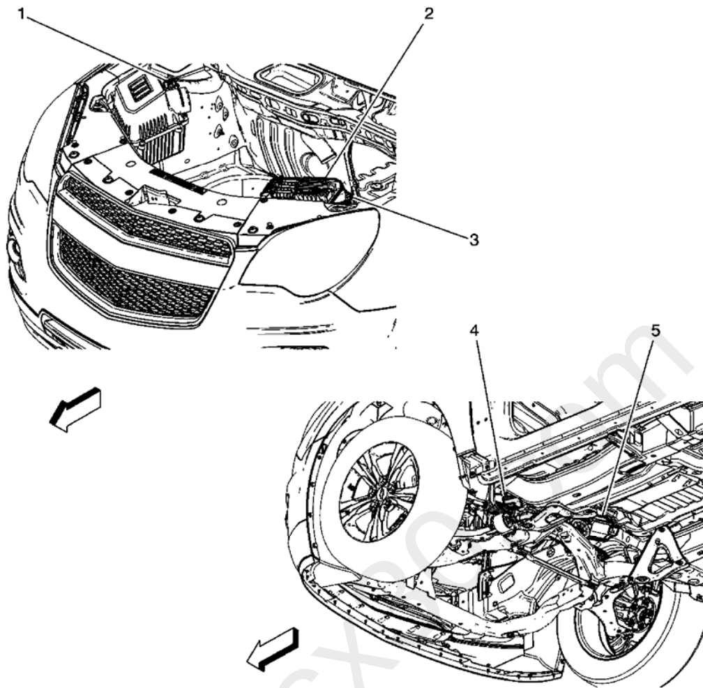
Fig. 3: Identifying Engine Compartment Components (Chevrolet) Courtesy of GENERAL MOTORS CORP.
